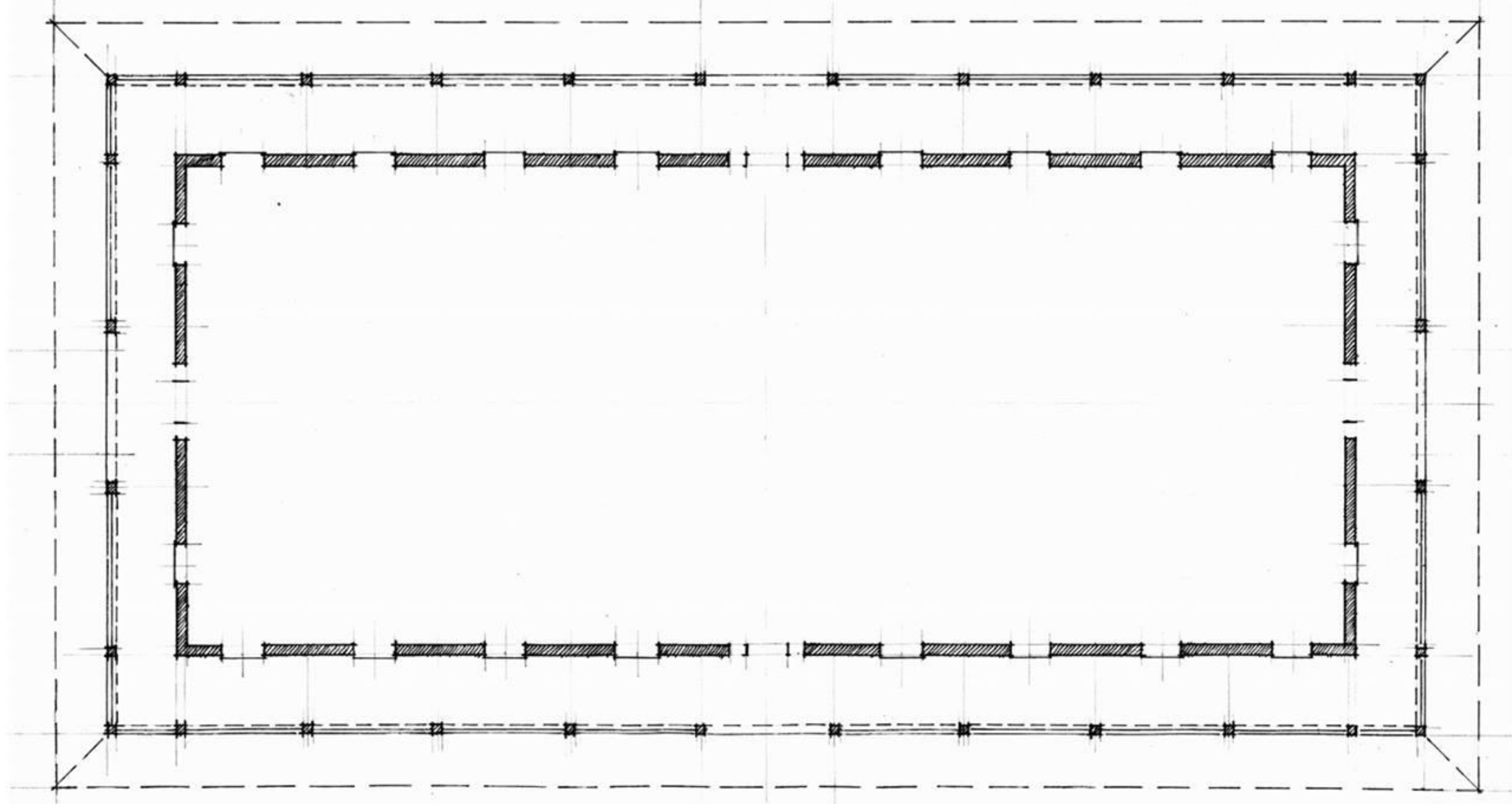
FLOOR PLAN
